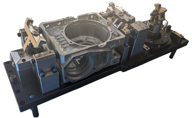
Alluminium Gear box 4TH AXIS FIXTURE
