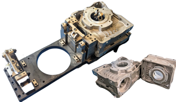
Alluminium Gear box 4TH AXIS FIXTURE
