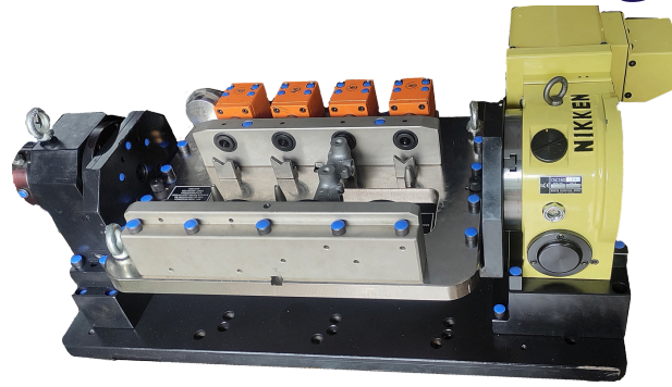
TANDEM MASTER CYLINDERS 4TH AXIS HYDRAULIC FIXTURE WITH CRADLE ARRANGEMENT
