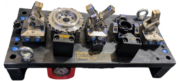
Boss Drilling Hyd. Fixture
