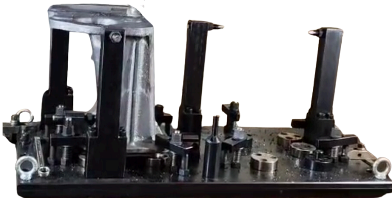
GB Mounting Bracket OP-20- 30 mechanical fixture
