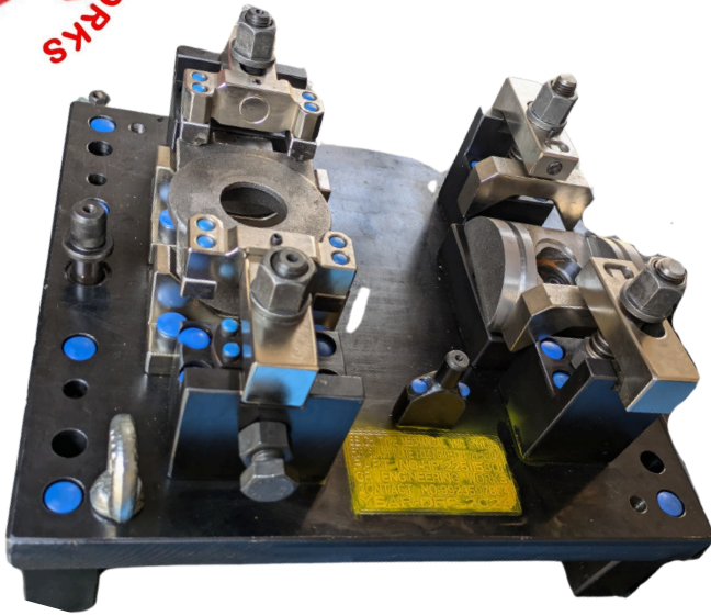
Swash Plate OP 20 mechanical fixture
