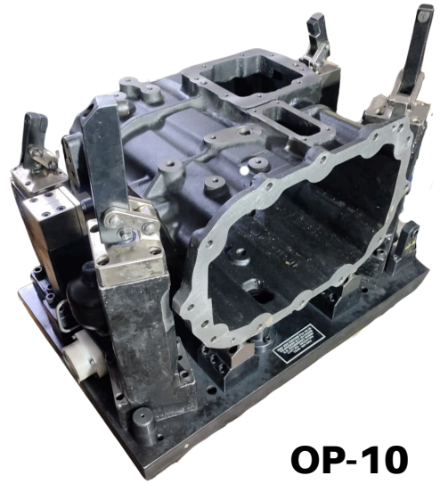
TM Case HMC Hydraulic Fixture
