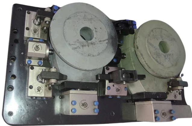
Gear Box DN series 4TH AXIS FIXTURE
