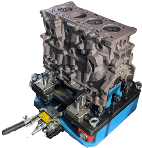
Engine Block HMC Hydraulic Fixture
