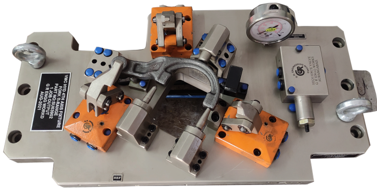
Fork 4TH AXIS FIXTURE
