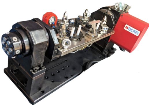
Gear box 4TH AXIS HYDRAULIC FIXTURE WITH CRADLE ARRANGEMENT
