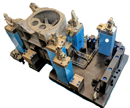
MS Gear box 4TH AXIS FIXTURE
