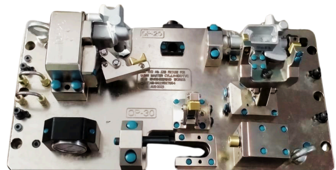
Master cylinder 4TH AXIS FIXTURE
