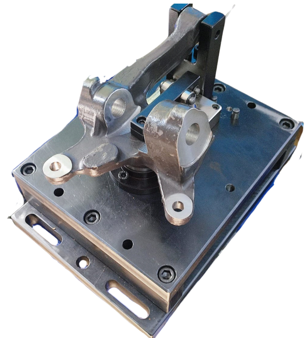
Knuckle joint Hyd. Fixture
