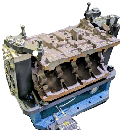
Engine Block HMC Hydraulic Fixture
