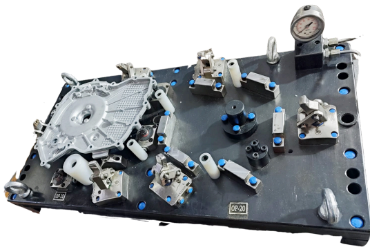
Side Cover Hyd. Fixture
