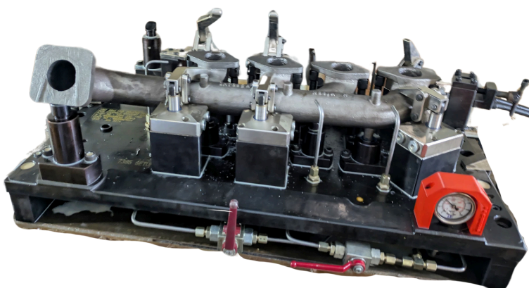
Exhaust Manifold OP 10 Hyd. Fixture
