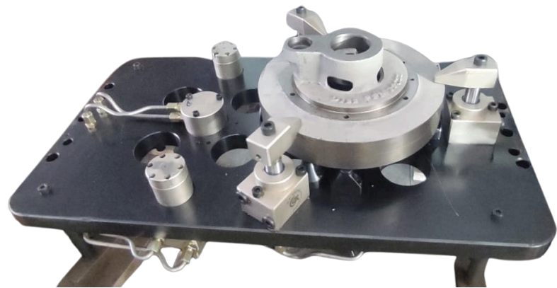
EV BATTERY COVER 4TH AXIS FIXTURE
