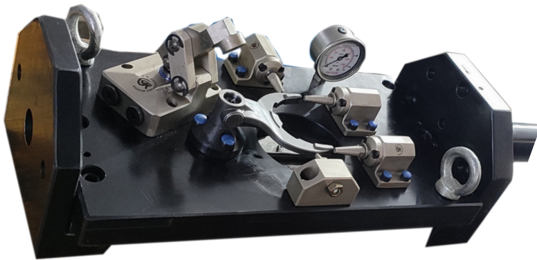
Fork 4TH AXIS FIXTURE
