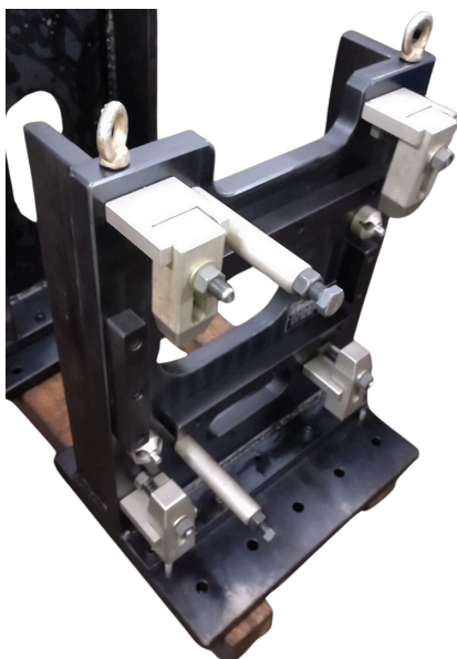
Clutch Housing HMC mechanical fixture
