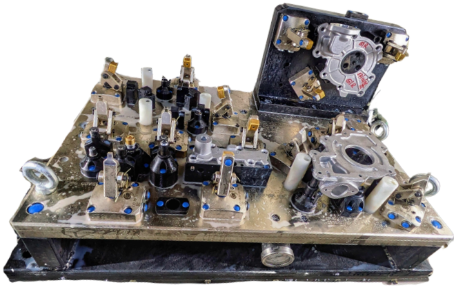
Side cover Hyd. Fixture
