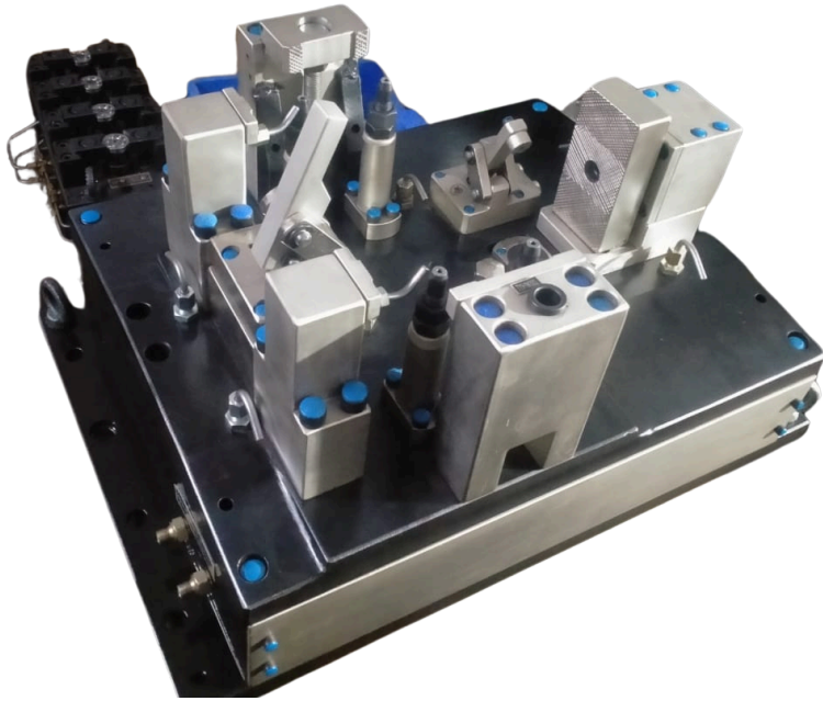
Navistar hyd. fixture
