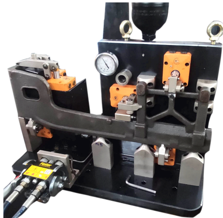
Bracket HMC Hydraulic fixture
