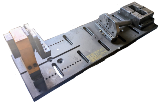
Gear box 4TH AXIS HYDRAULIC FIXTURE WITH CRADLE ARRANGEMENT
