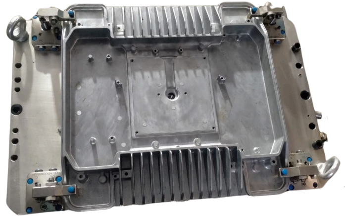
EV BATTERY COVER 4TH AXIS FIXTURE
