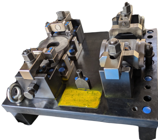
Swash Plate mechanical fixture
