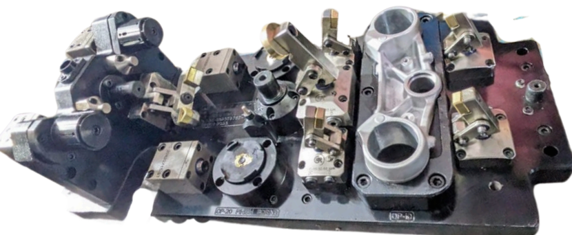
HMCL under bracket 4TH AXIS FIXTURE
