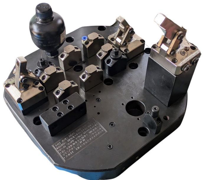
EGR Mixer 5 Axis Hydraulic fixture
