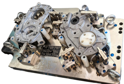
Oil pump cover 4Th axis fixture
