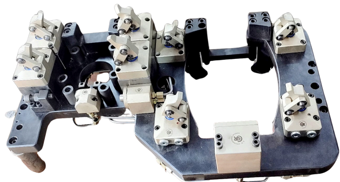
Gear Box 4TH AXIS FIXTURE
