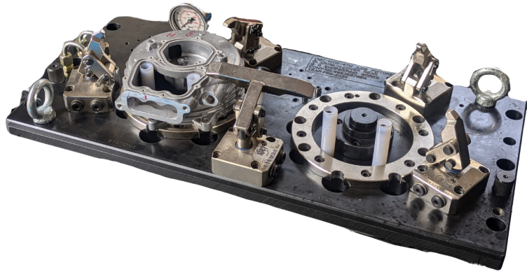
Electric motor cover 4TH AXIS FIXTURE
