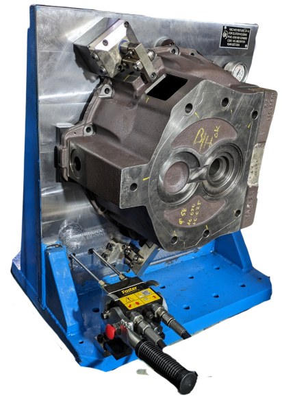
Clutch Housing HMC Fixture
