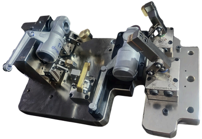
Axel Clamp 4TH AXIS FIXTURE
