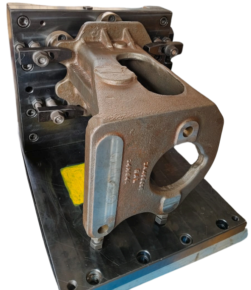
Bracket HMC mechanical fixture
