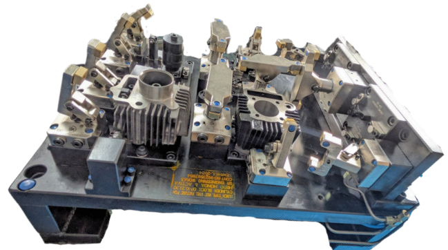
single cylinder engine block hyd. fixture
